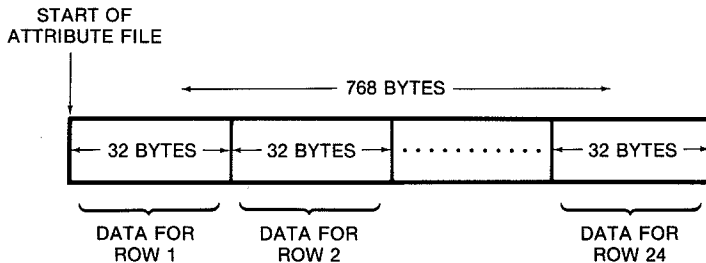
Fig. 8-7. Attribute file organization. (Courtesy Timex Computer Corp.)
